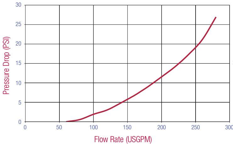
J72 Pressure Drop
